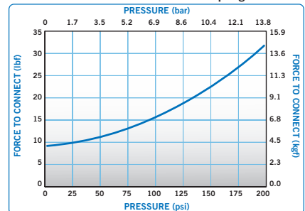
PLQ2 Force to Connect Coupling
